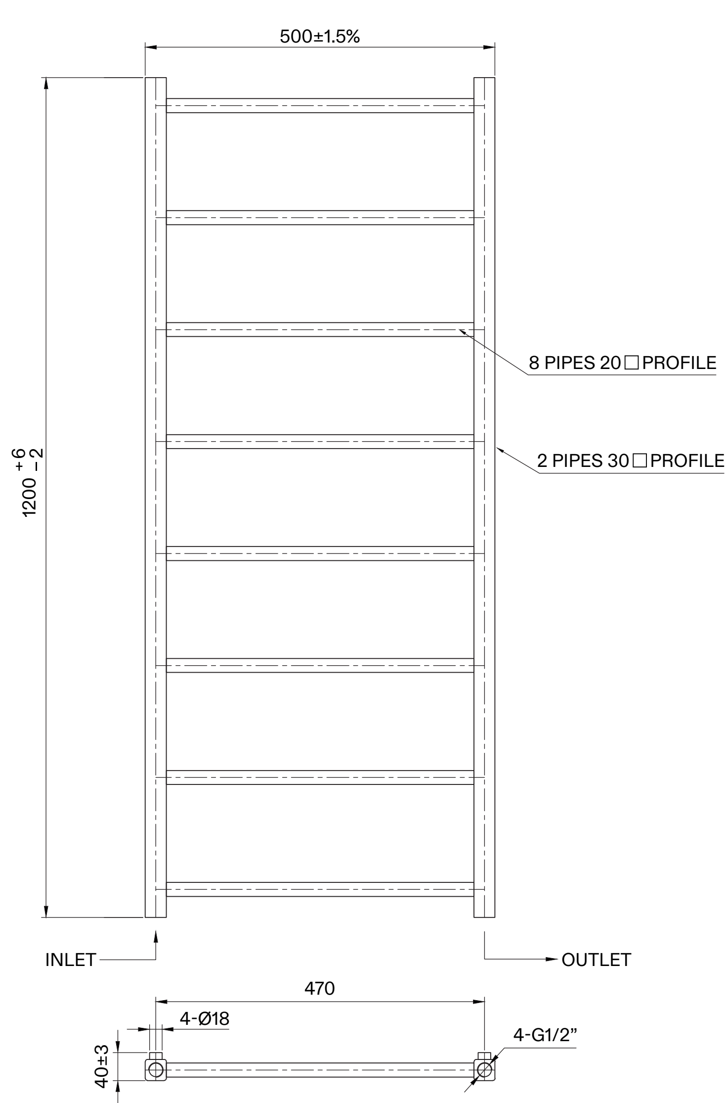
Front View
