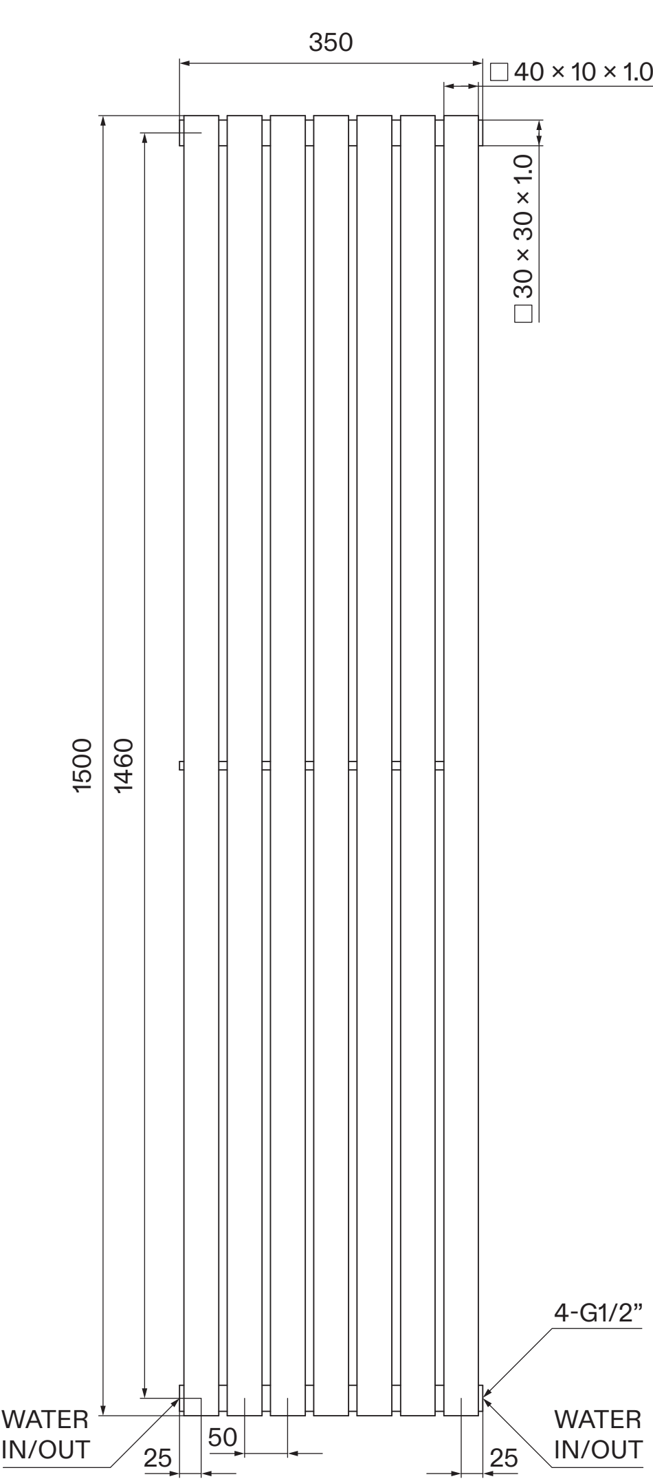
Front View
