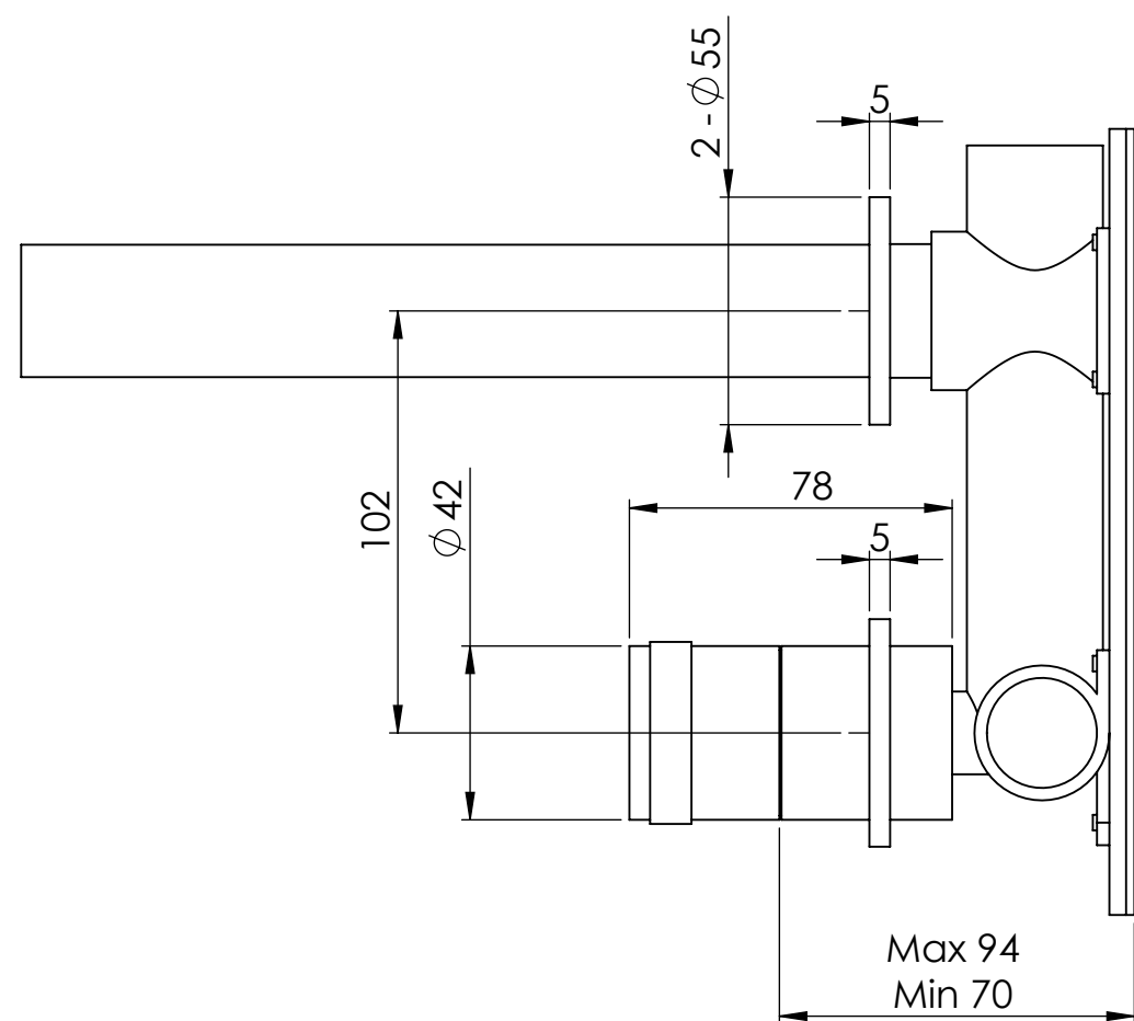
Top View
