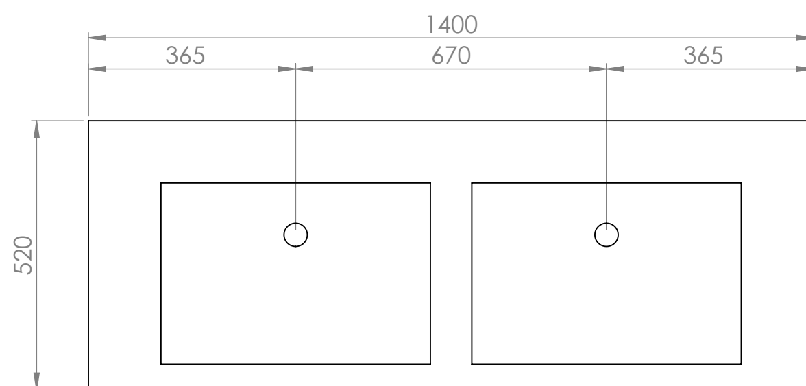
Top View
