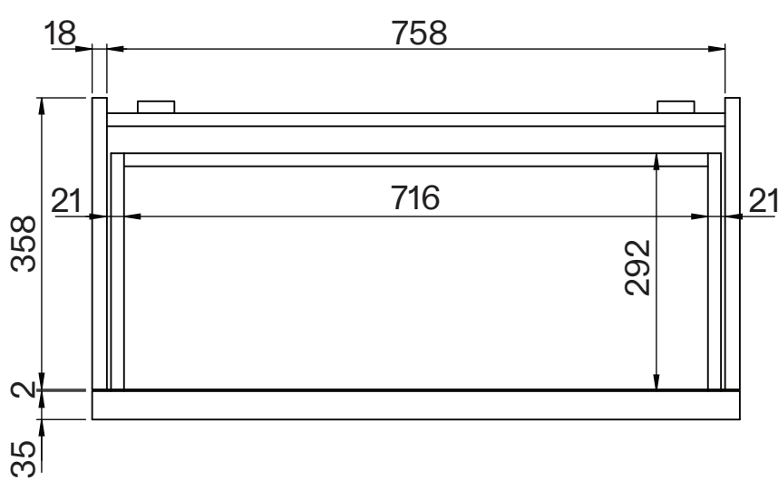
Top View - Section View
