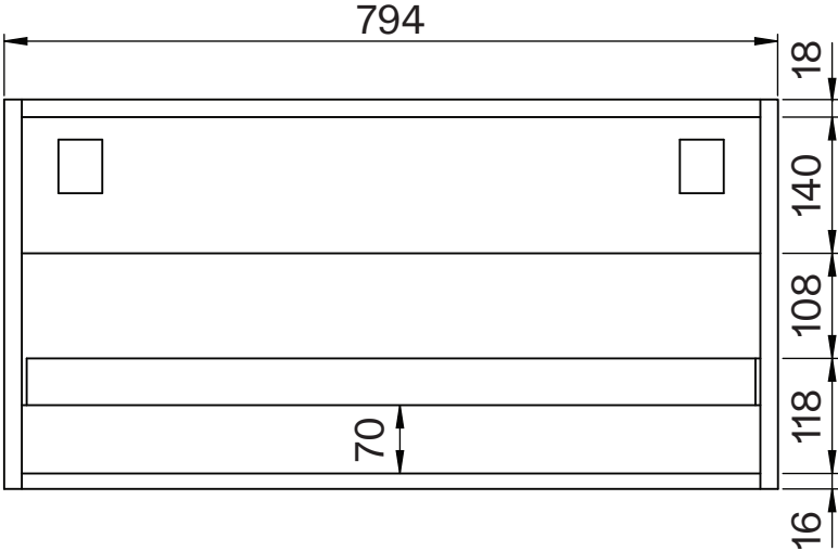
Back View - Cabinet
