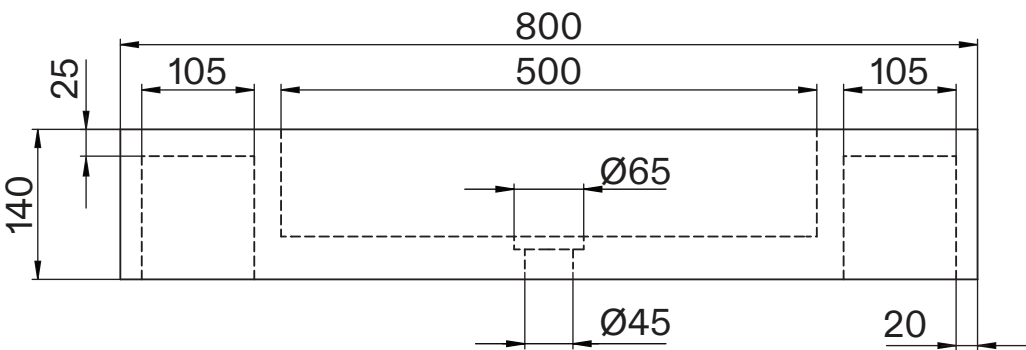
Front View - Section View
