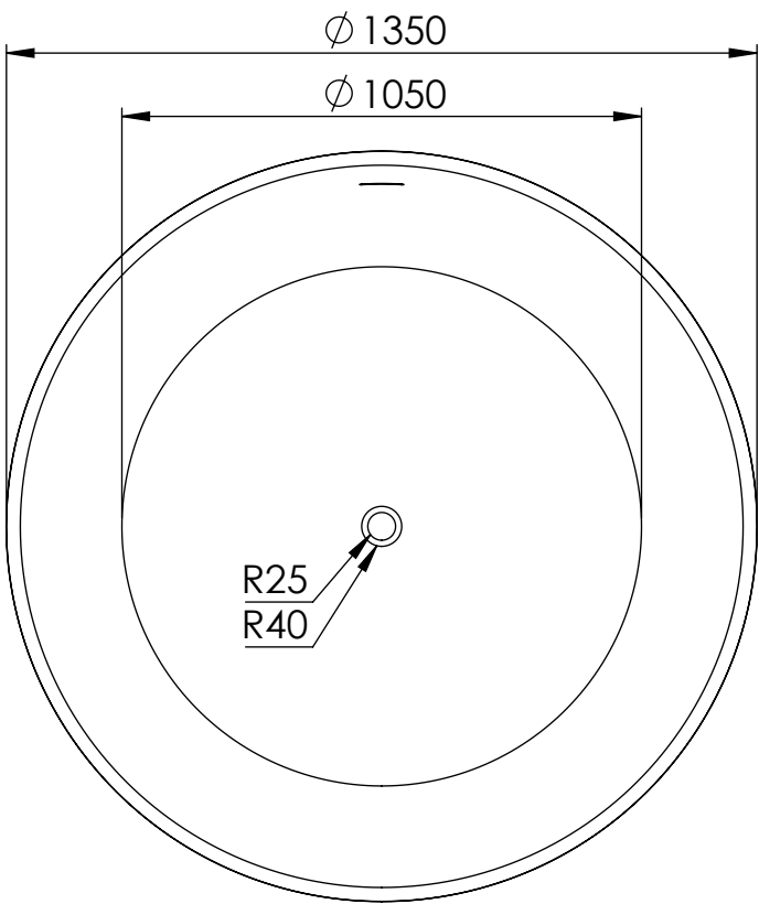
Top View
