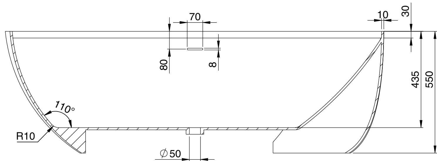
Front View - Section View
