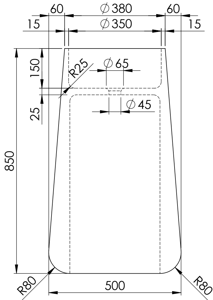
Front View - Section View
