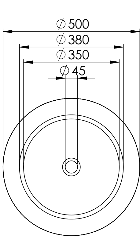
Top View
