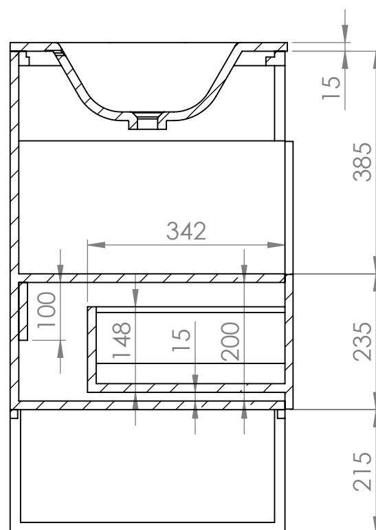
Side View - Section View
