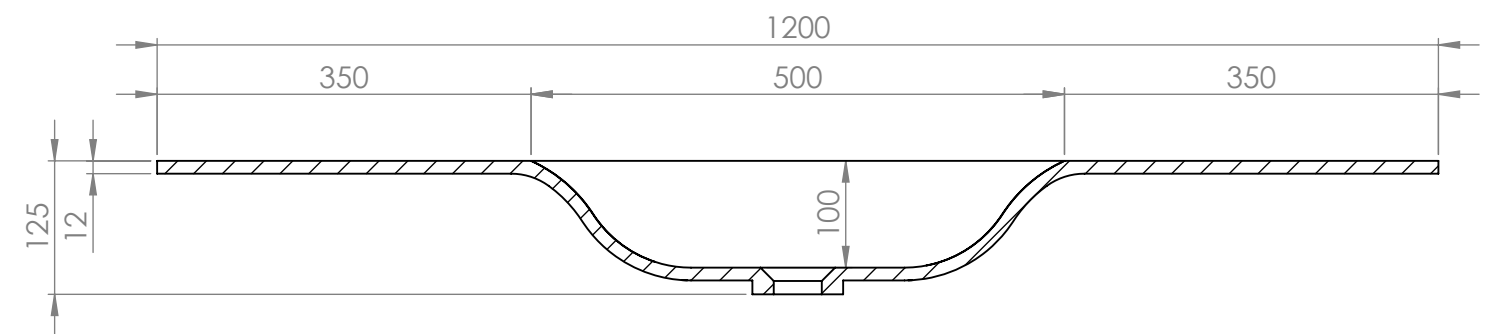
Side View - Section View
