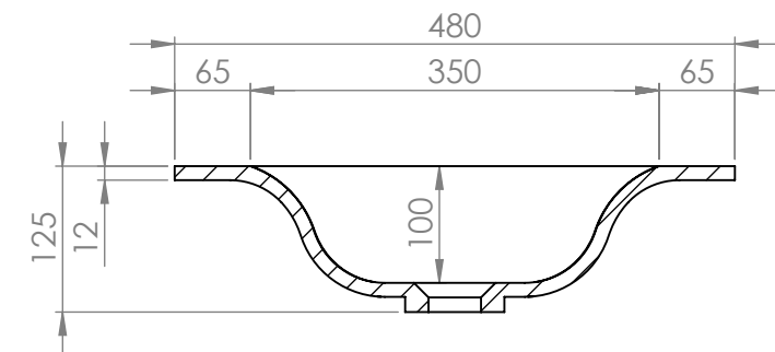
Side View - Section View
