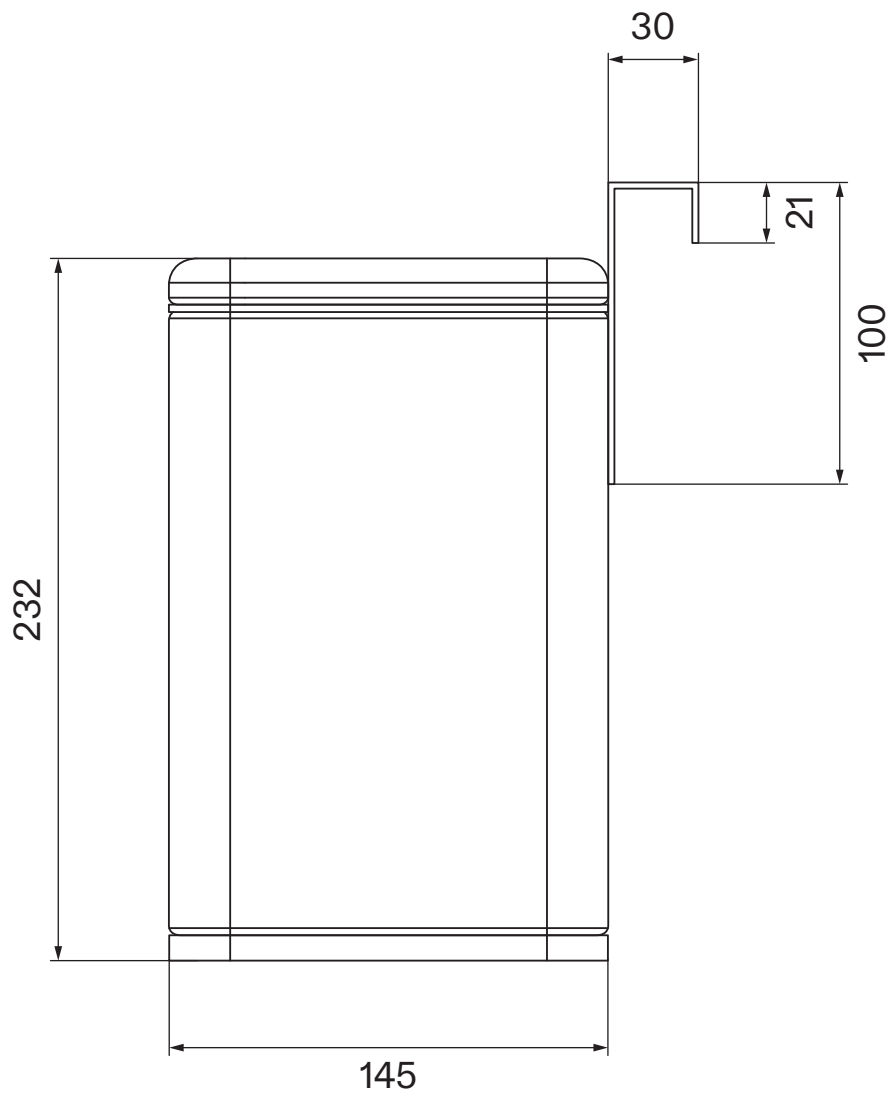
Side View
