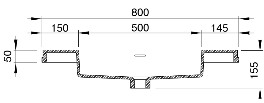
Basin - Section View Front View
