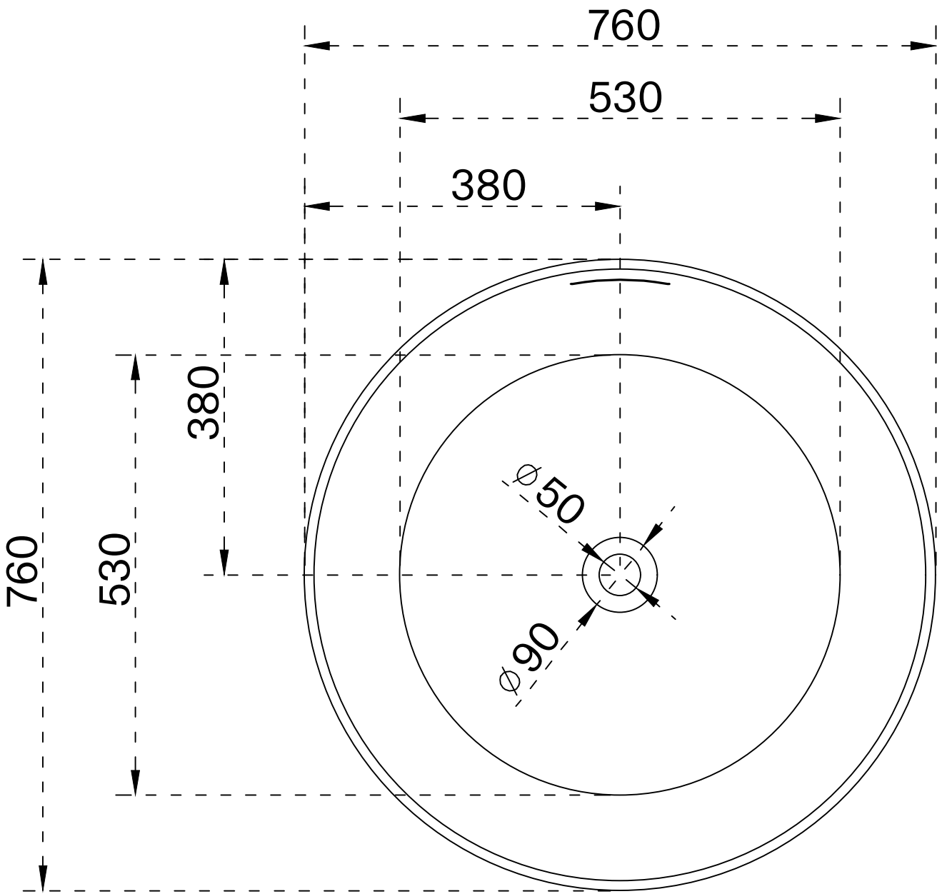
Top view
