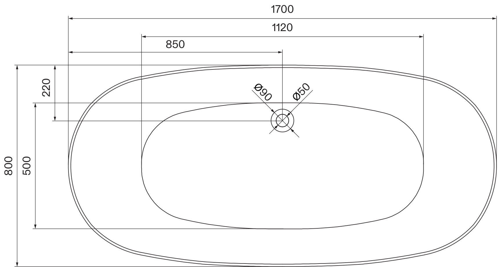
Top View
