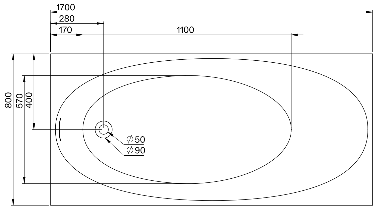
Top View
