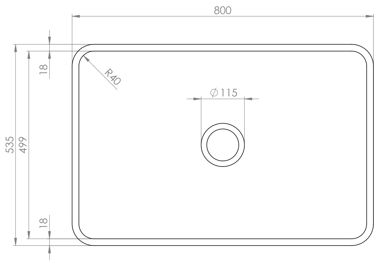
Top View
