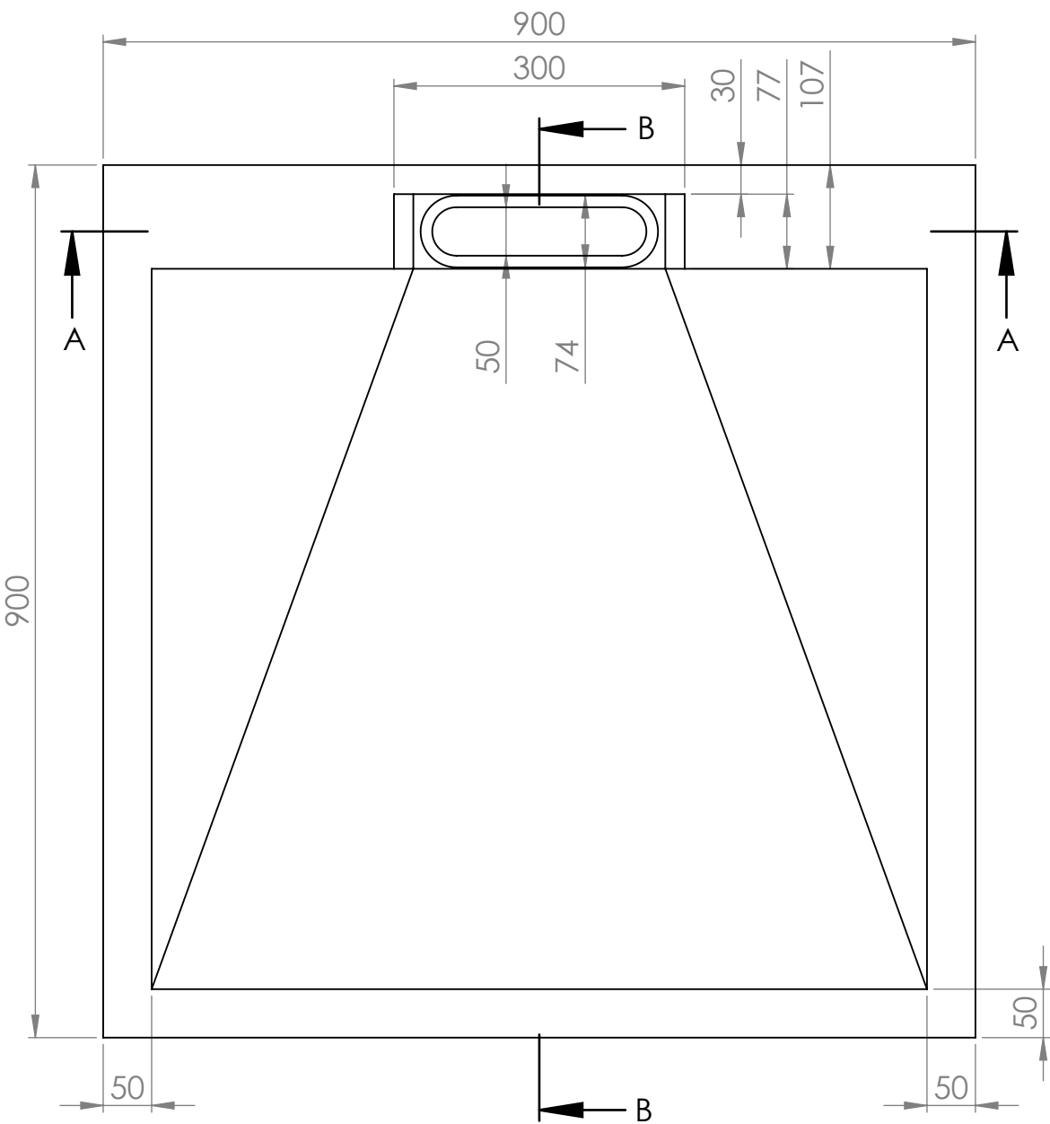
Top View
