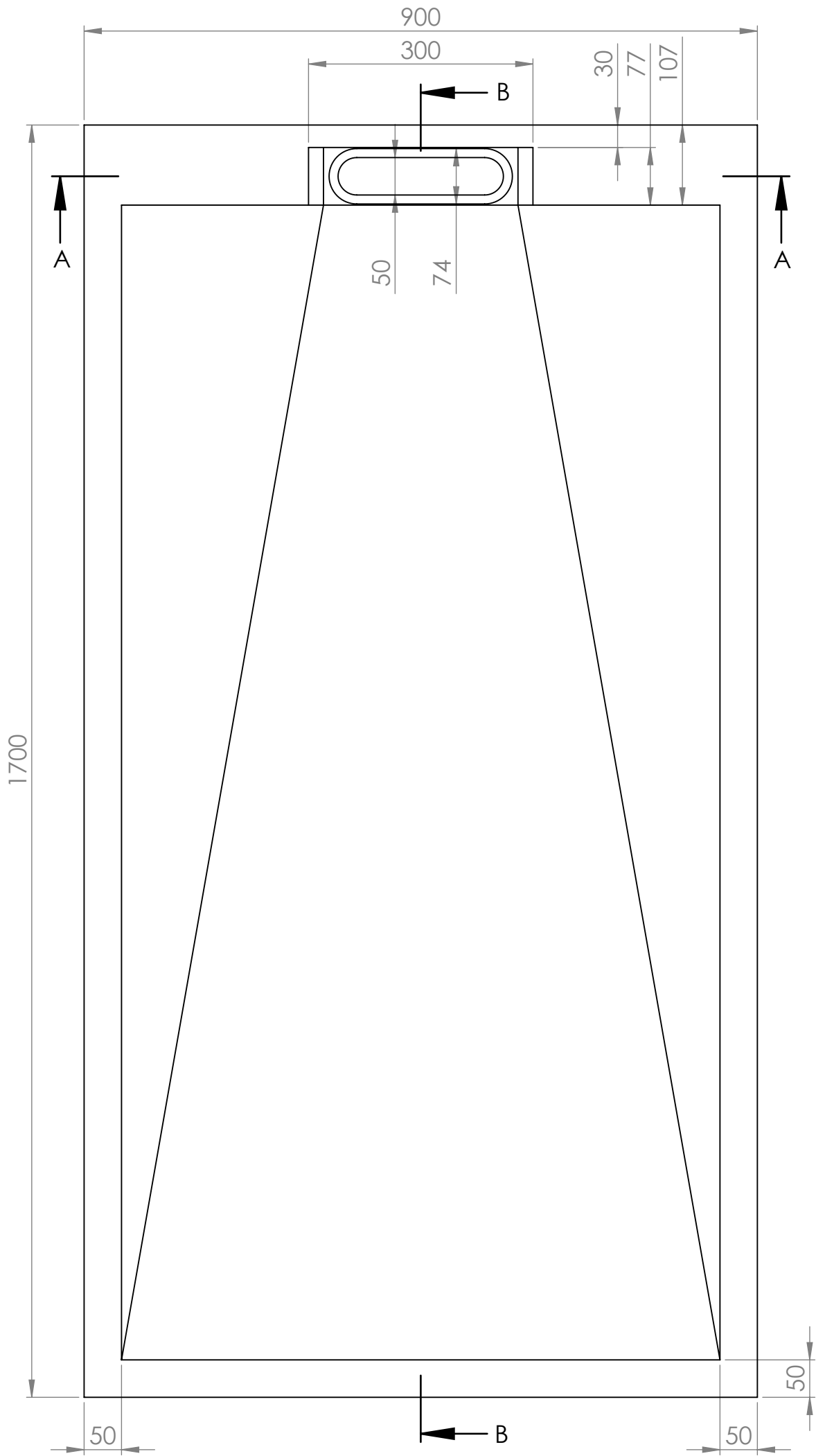
Top View
