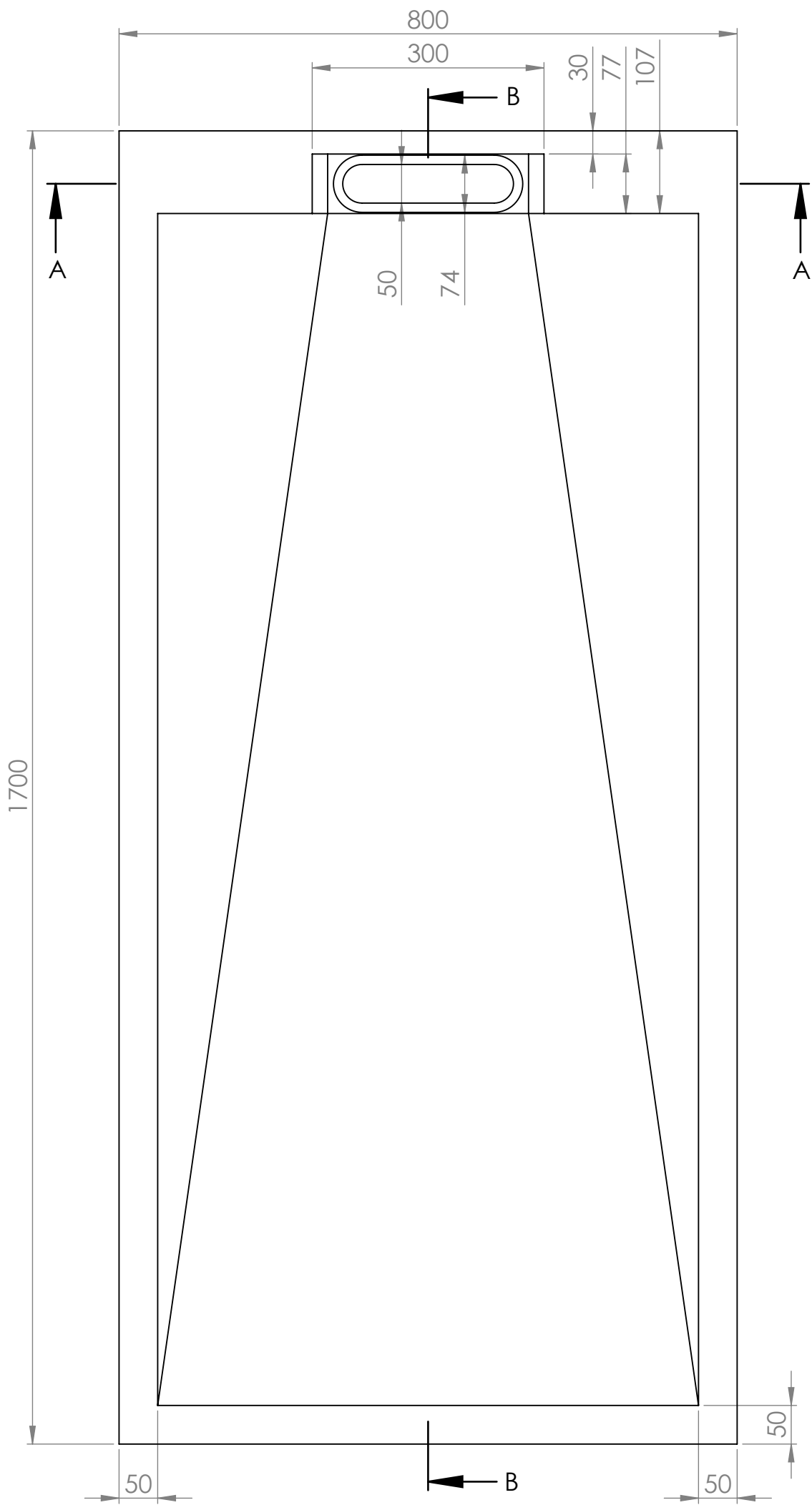
Top View
