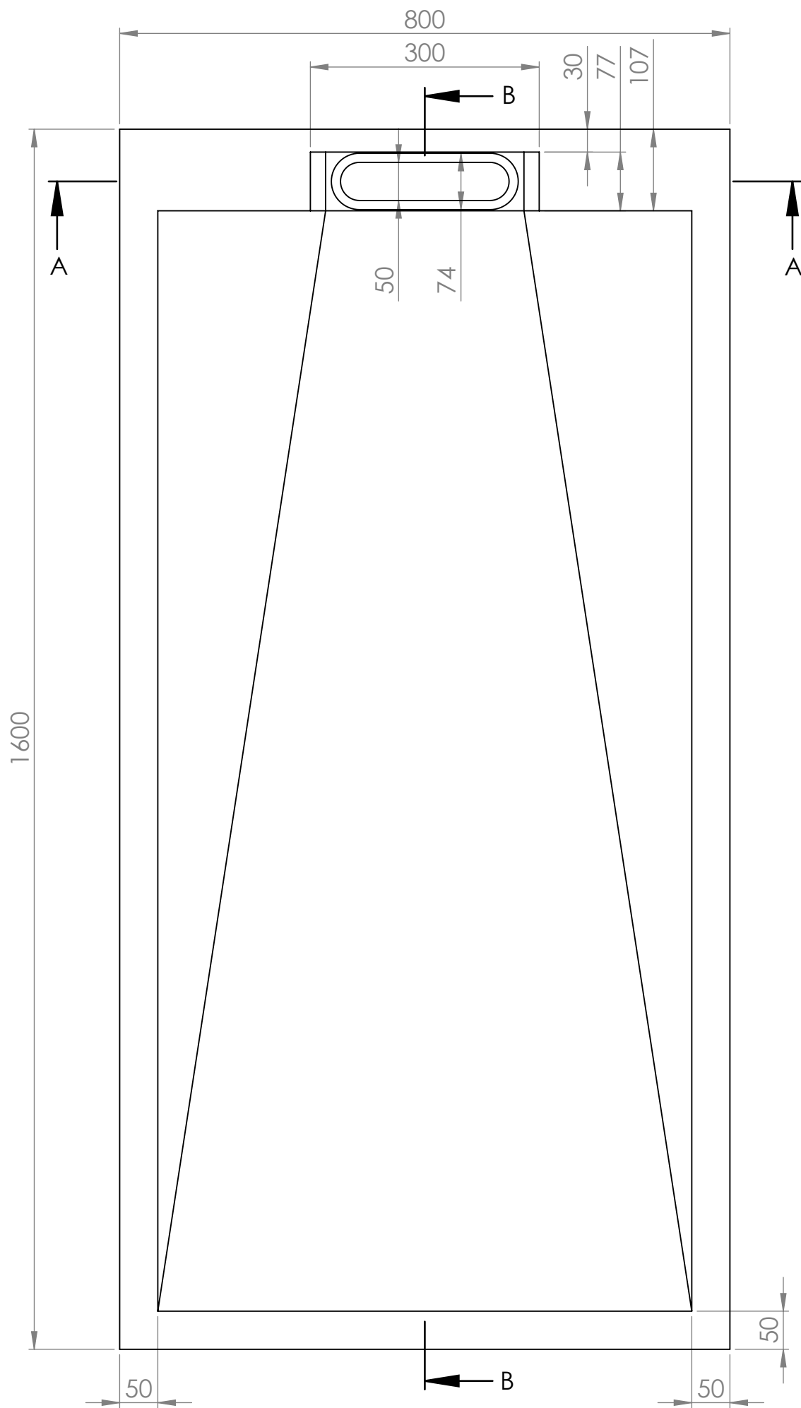
Top View
