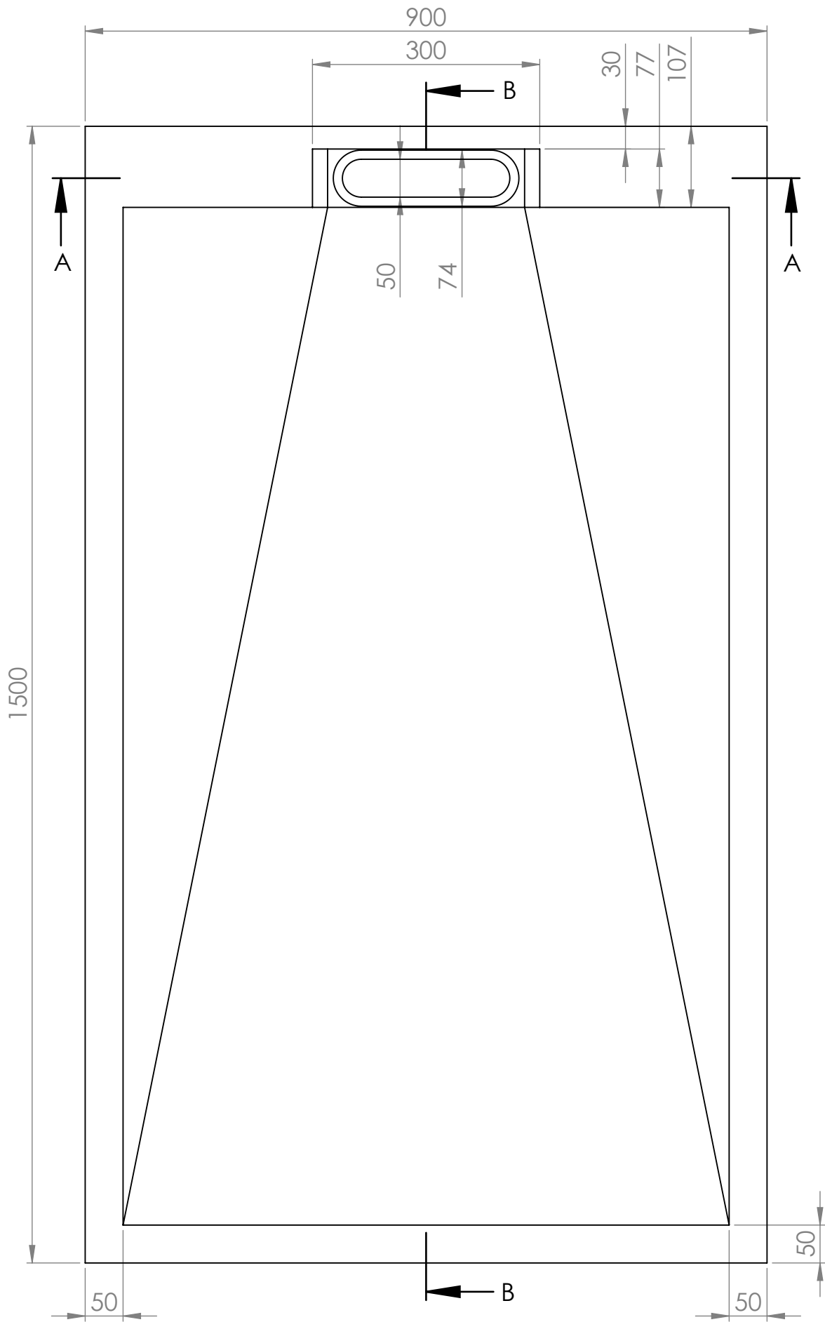
Top View
