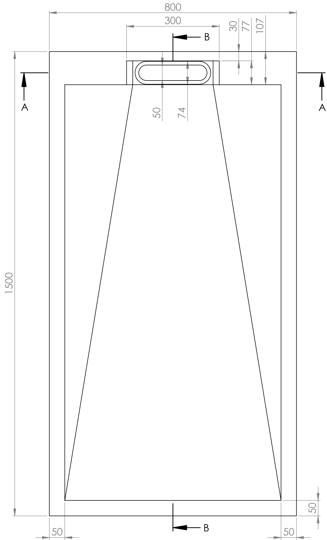
Top View
