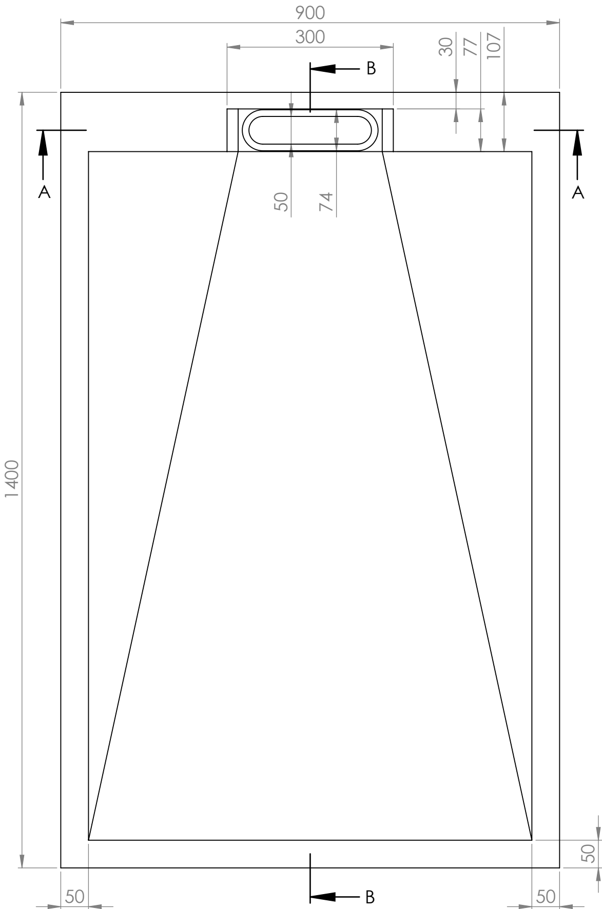
Top View
