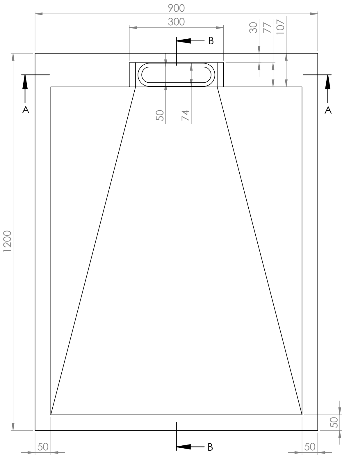
Top View
