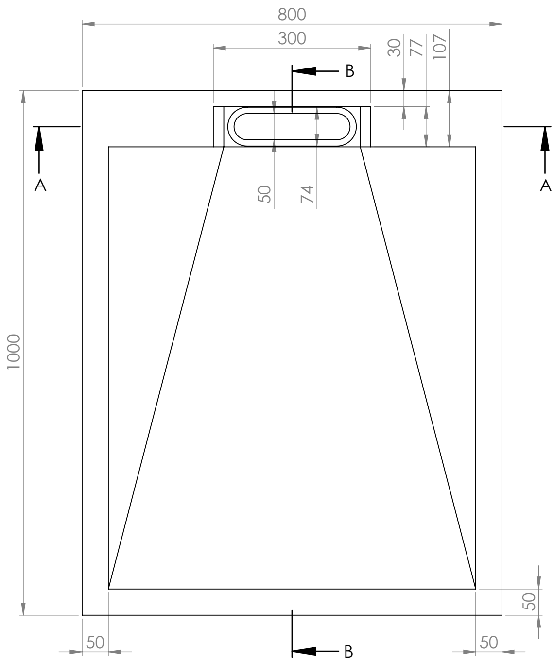
Top View
