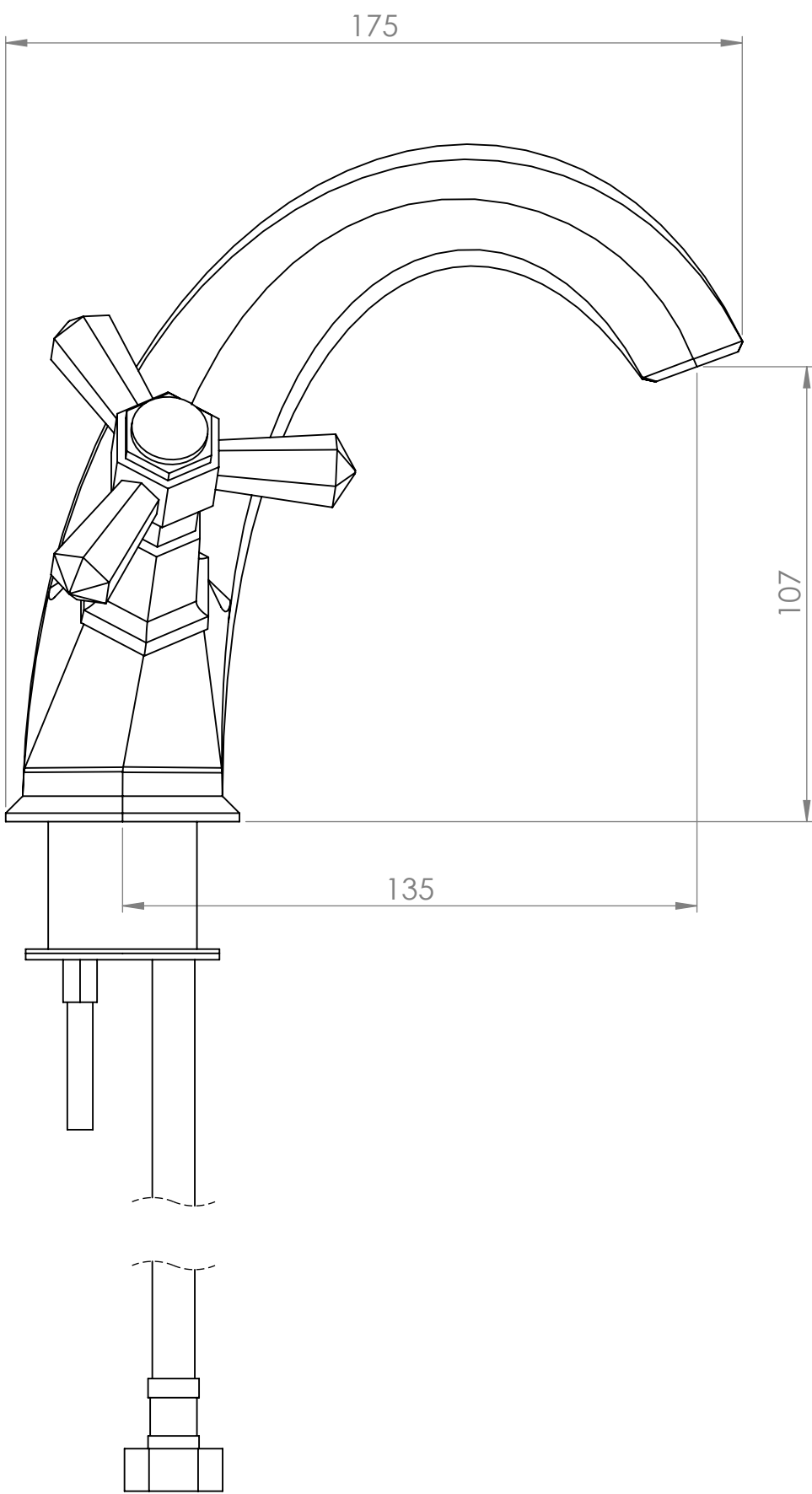
Side View
