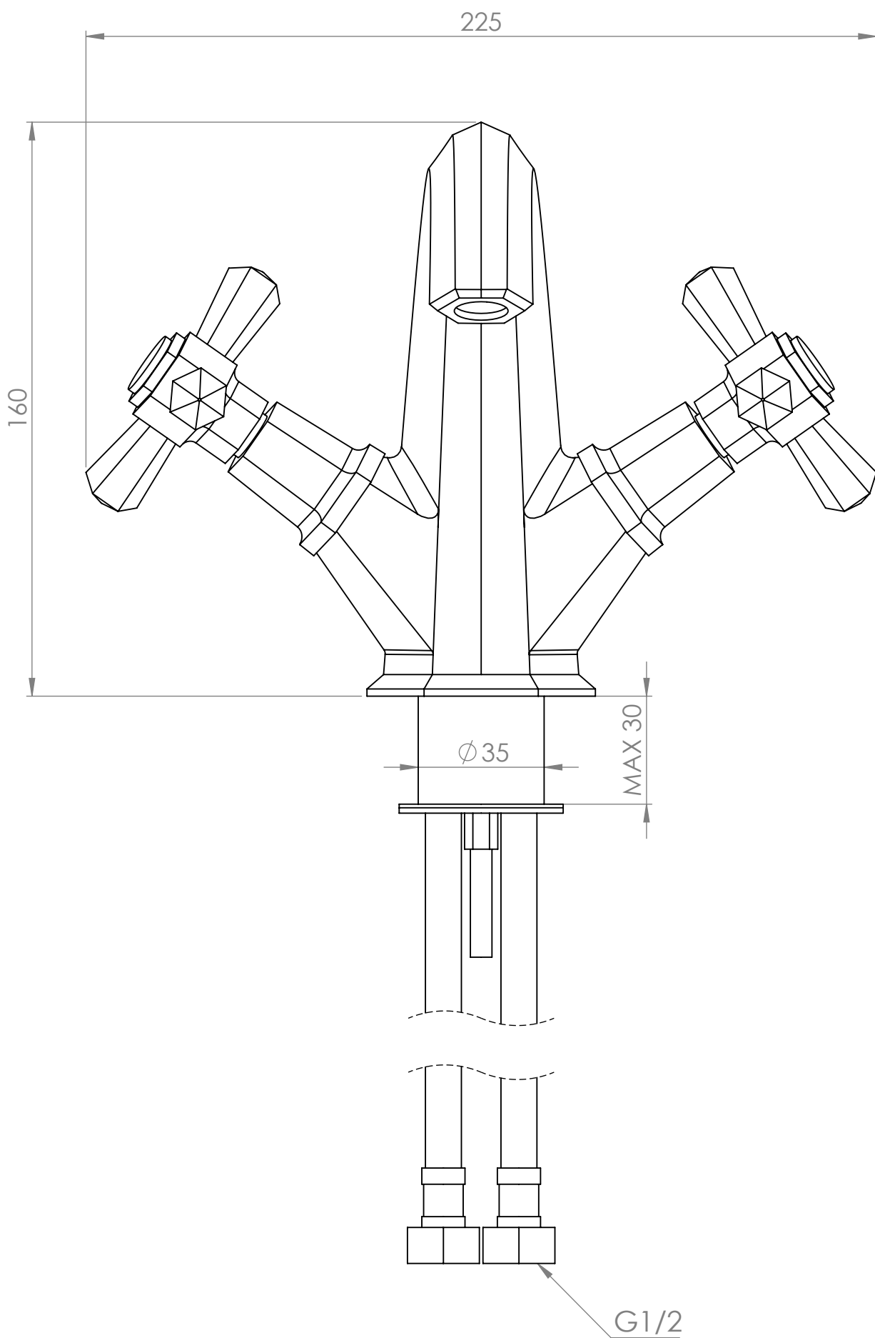
Front View
