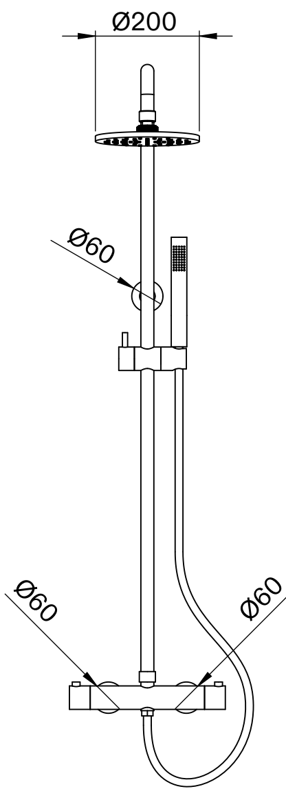
Front View
