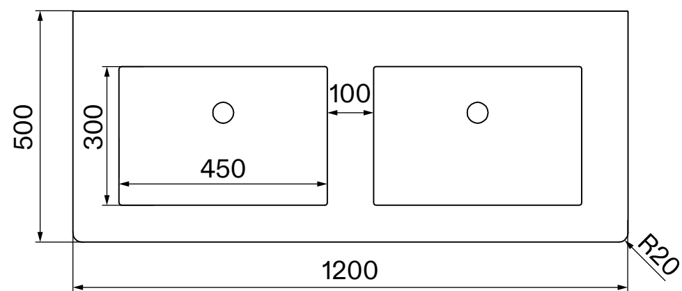
Top View
