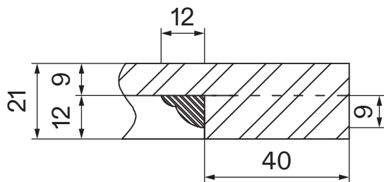
A-A - Section View
