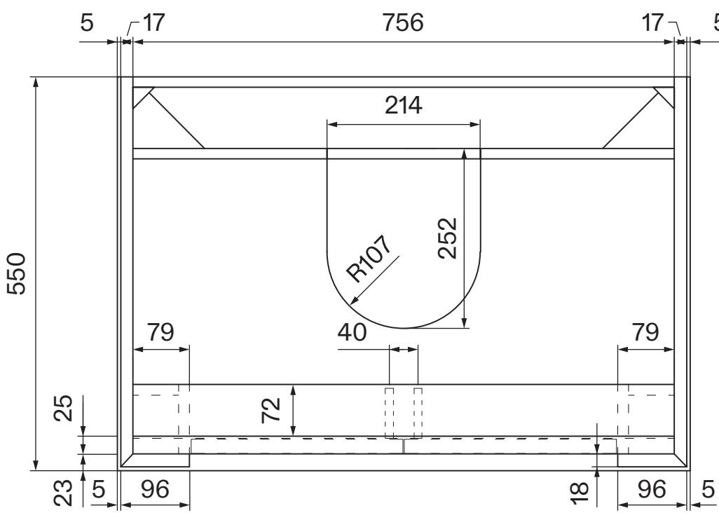
Bottom View
