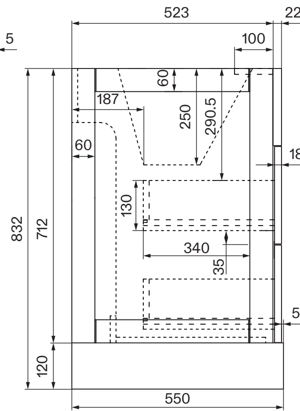
Side View
