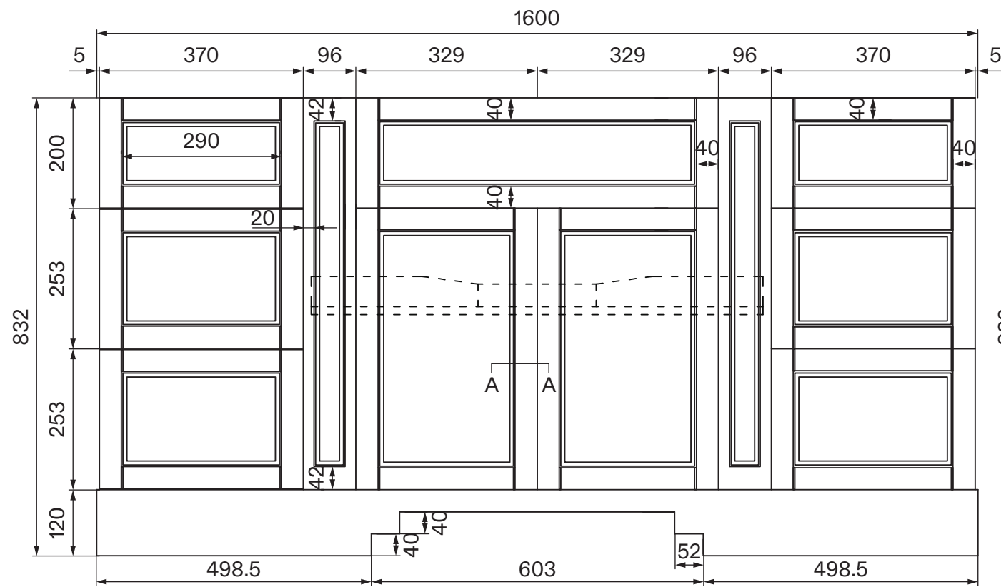
Front View
