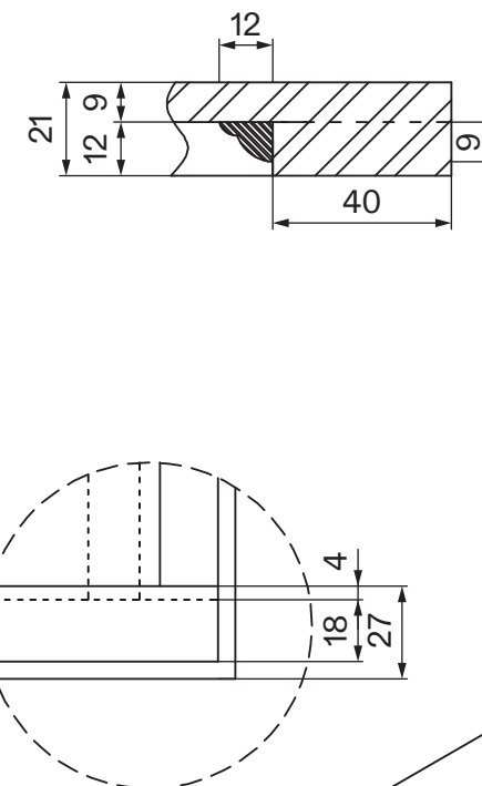
A-A - Section View
