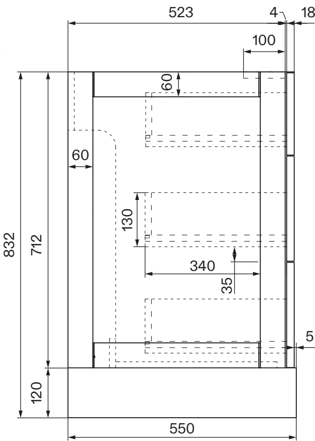
Side View
