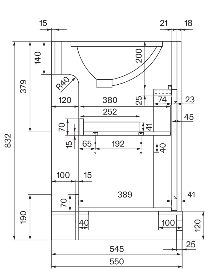
Side View - Section View
