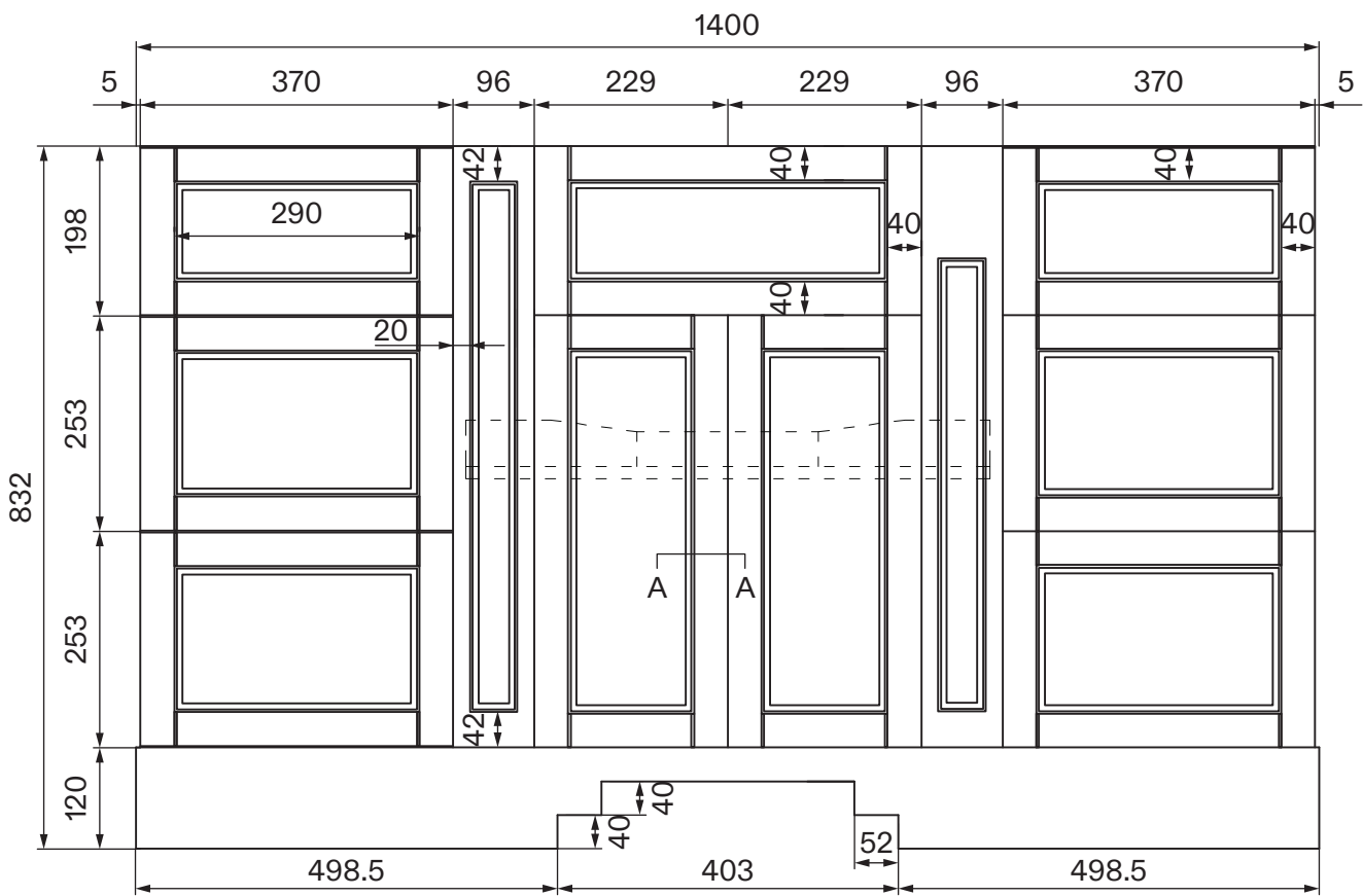
Front View
