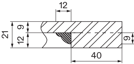
A-A - Section View
