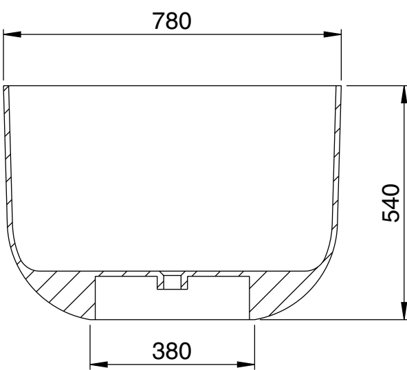
Side View - Section View
