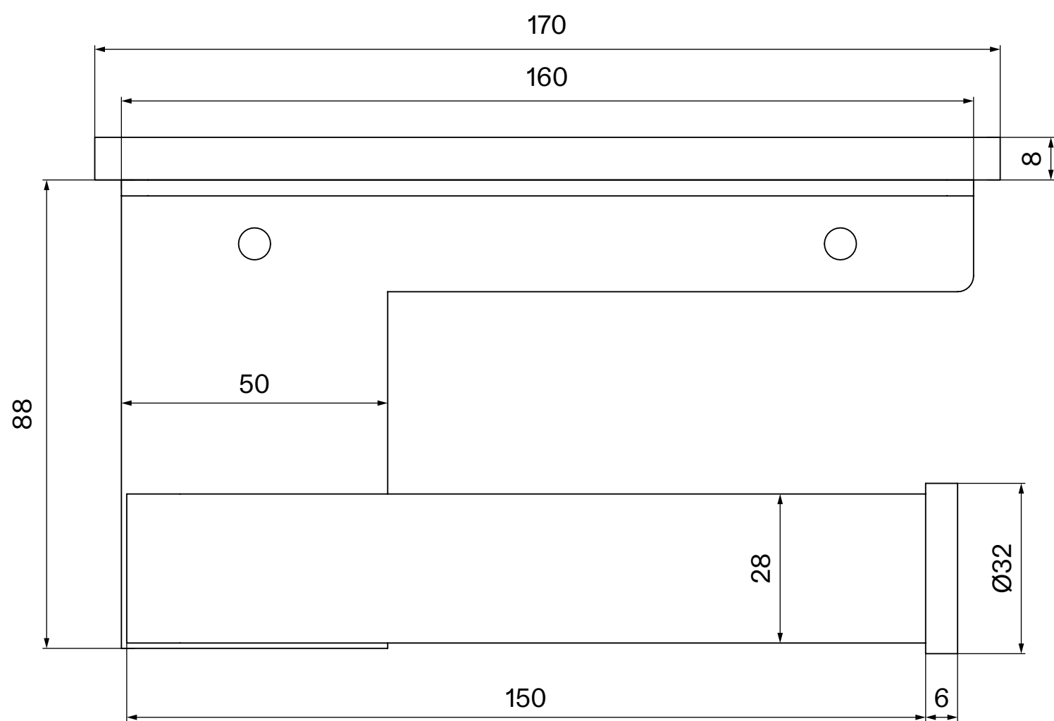
Top View
