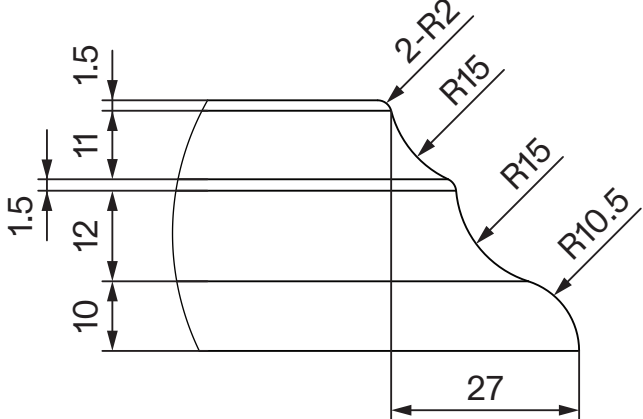
Detail A
