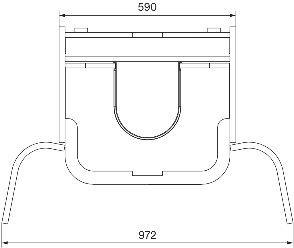
Side View
