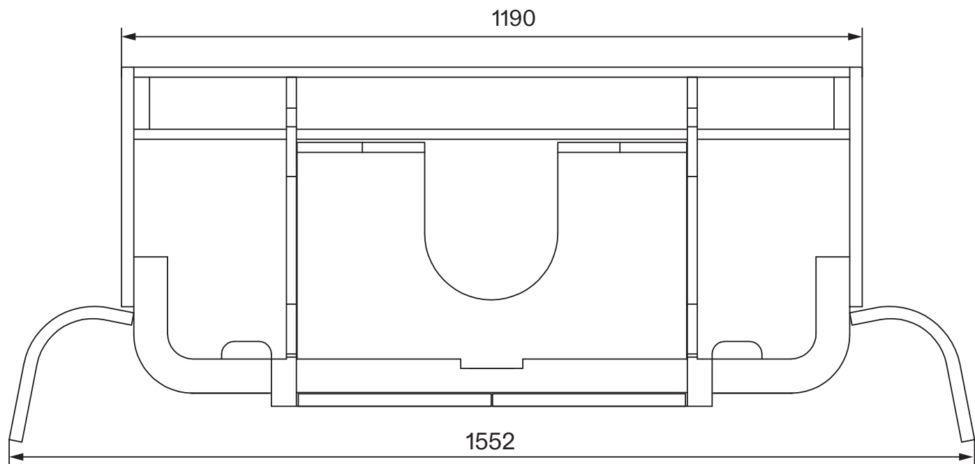
Bottom View
