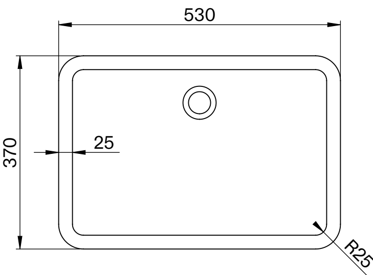
Basin - Top View
