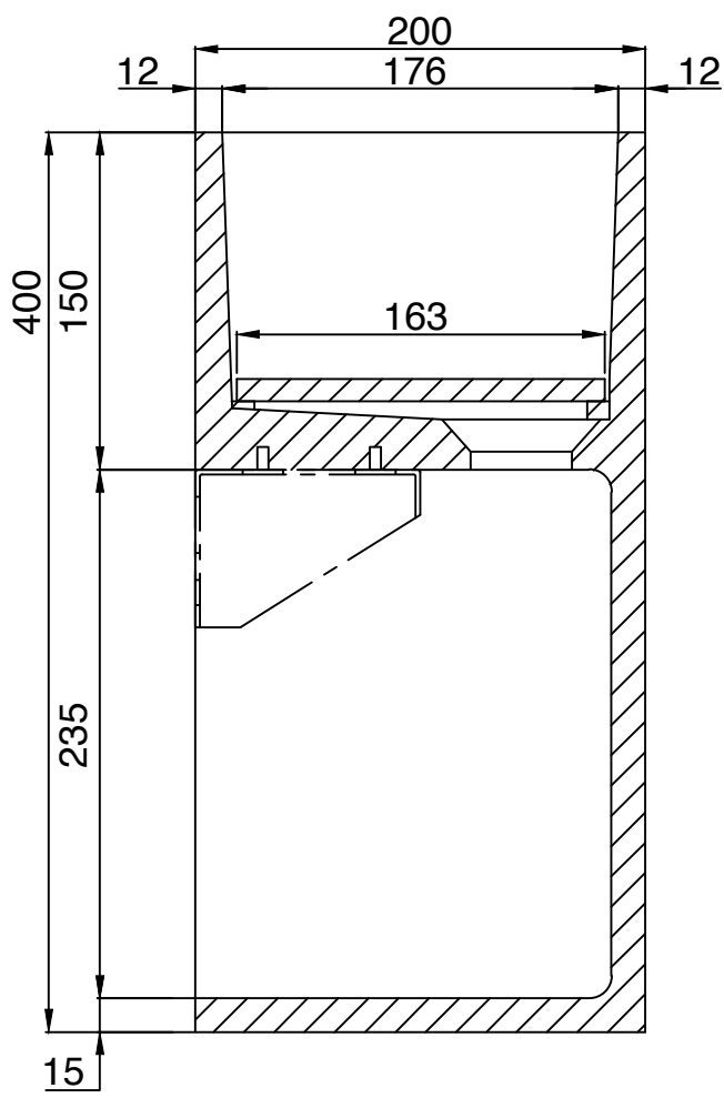
Side View - Section View
