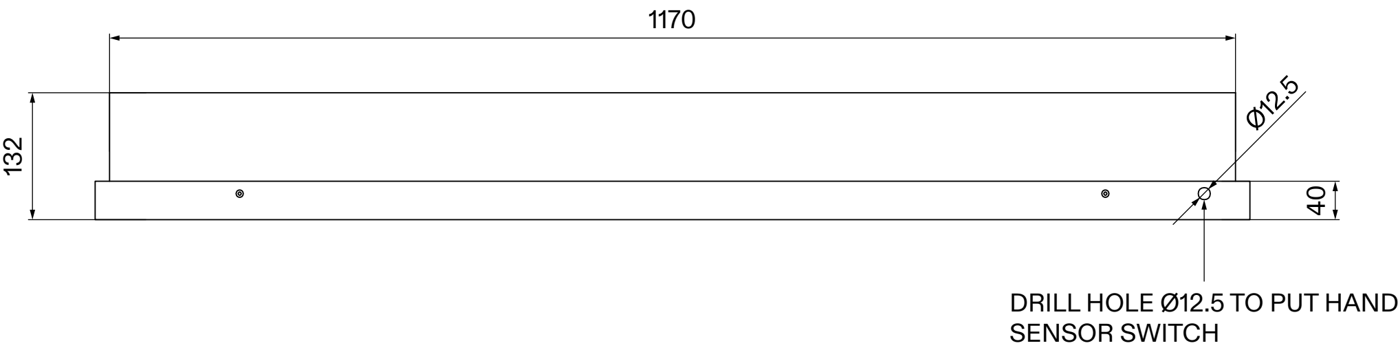
Bottom View
